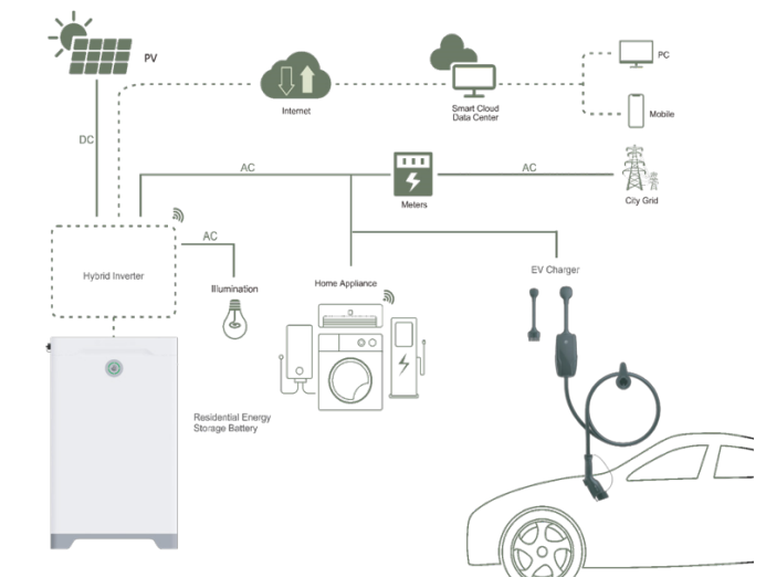
Operating Diagram of Residential Energy Storage System
